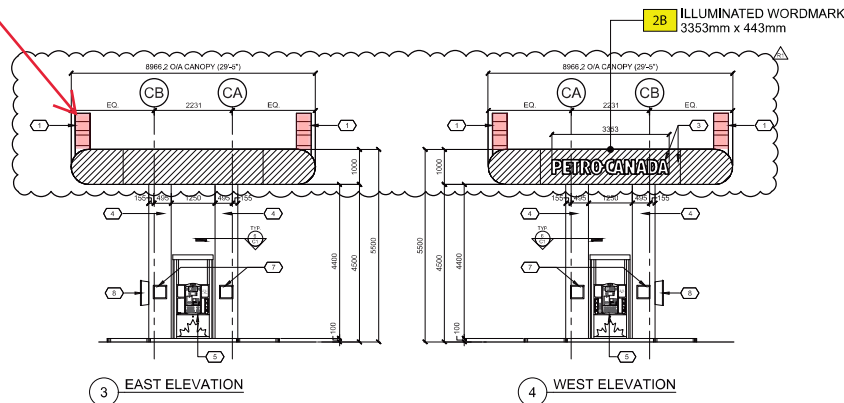
3 EAST ELEVATION
