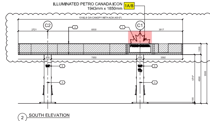
2 SOUTH ELEVATION
