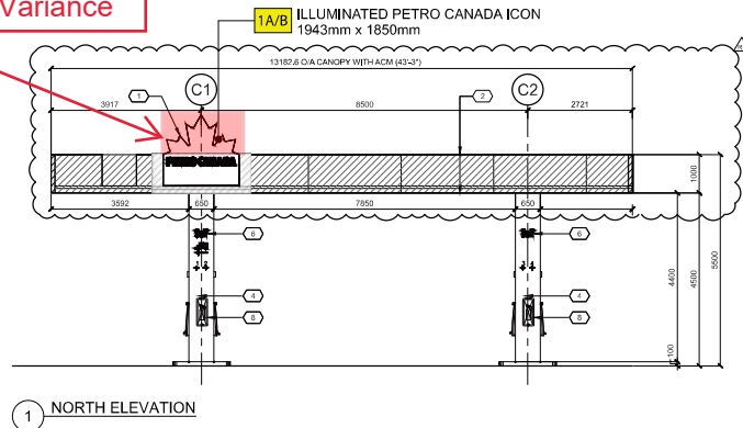
1 NORTH ELEVATION
