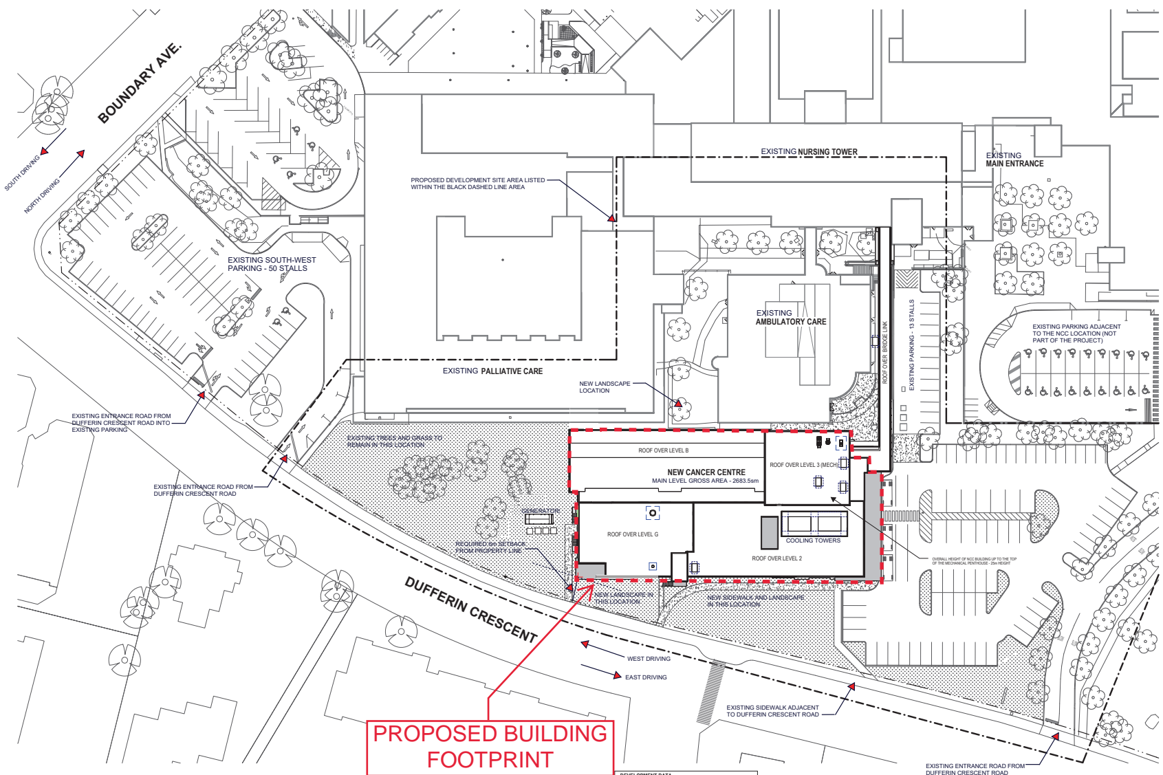
1 OVERALL SITE PLAN A101 1:200
