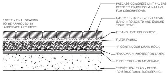
4 UNIT PAVING OVER SLAB L3 SCALE: 1-1/2" = 1' - 0"
