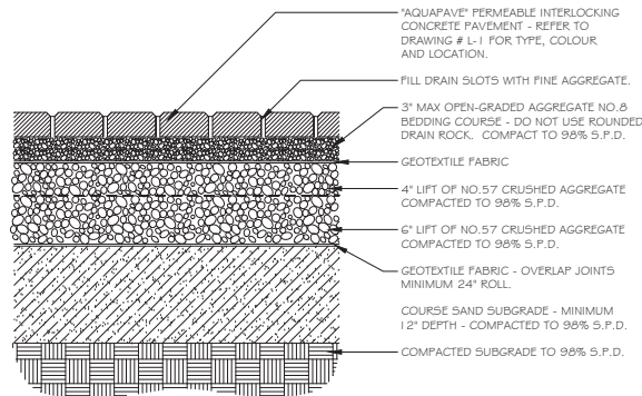
5 PERMEABLE PAVING L3 SCALE: 1-1/2" = 1' - 0"
