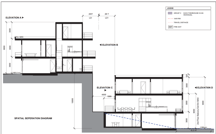
4 Townhome sections 1 : 100
