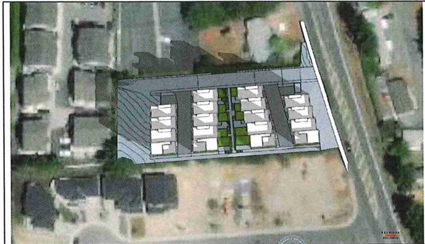
5915 METRAL DRIVE SHADOW STUDY - EQUINOX 9:00 am HANNAHO, NC SCALE: NTS 20' = 1" = 0'
