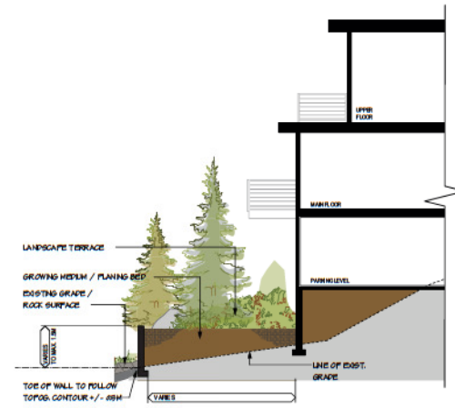
CONCEPTUAL LANDSCAPE TERRACE DETAIL
