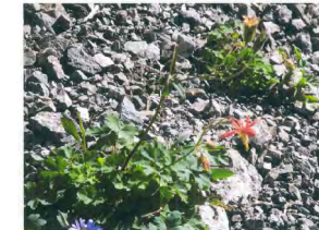
Scree slopes - angular rock colonized by plants
