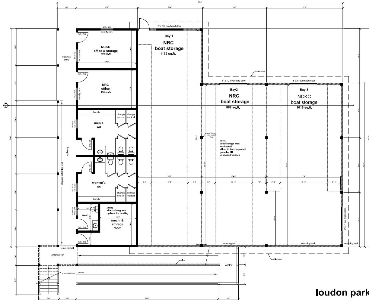
A2 lower level plan
