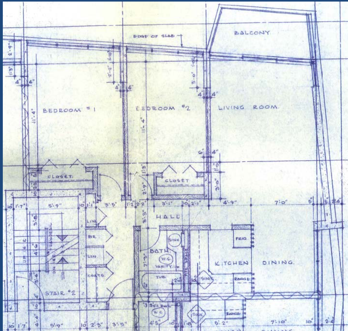
Original layout of two-bedroom apartment.
