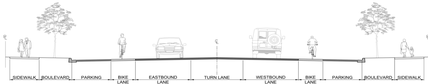
TYPICAL ROAD CROSS-SECTION
